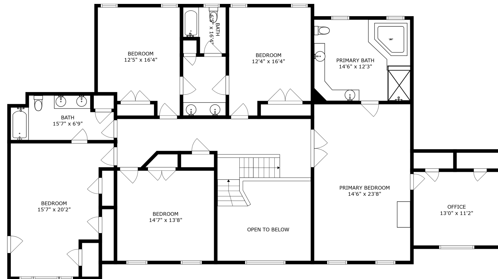
FLOOR 3
