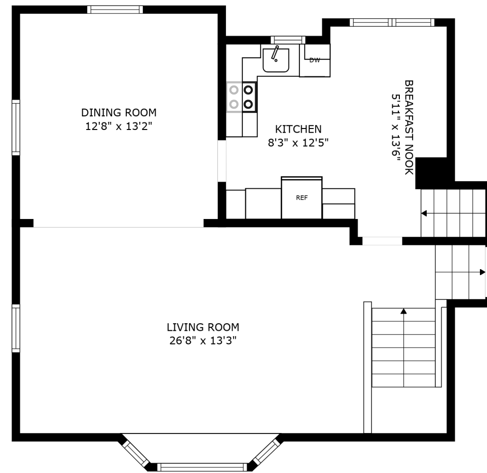
FLOOR 3
