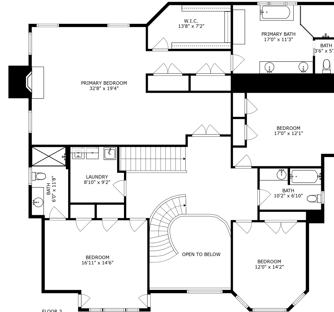
FLOOR 3
