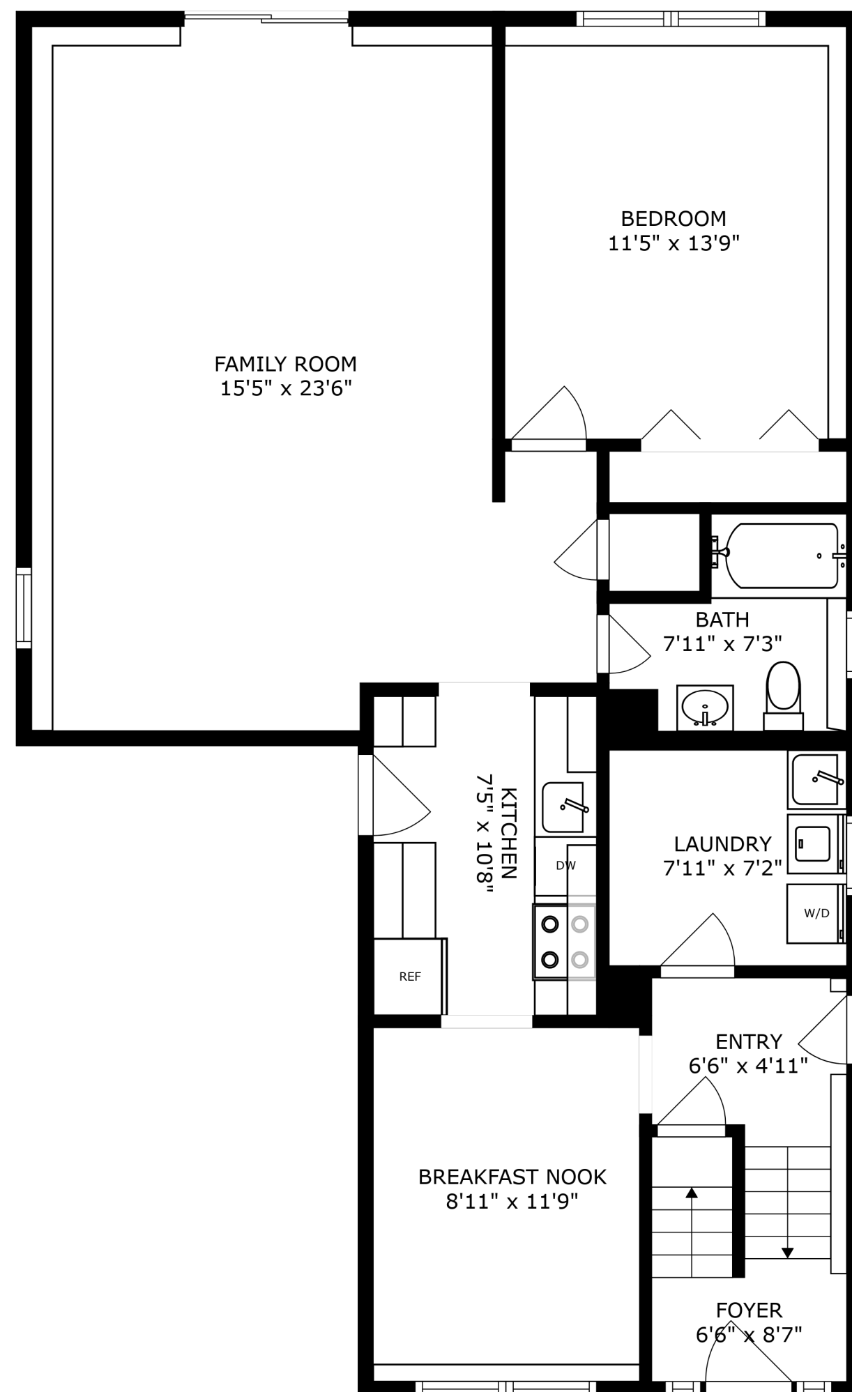
FLOOR 1
