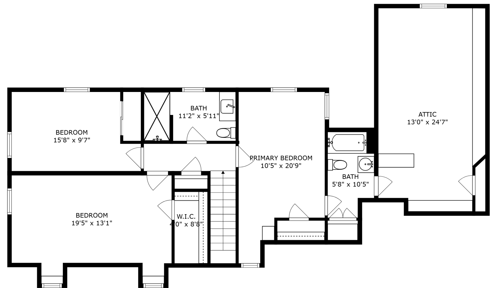
FLOOR 3
