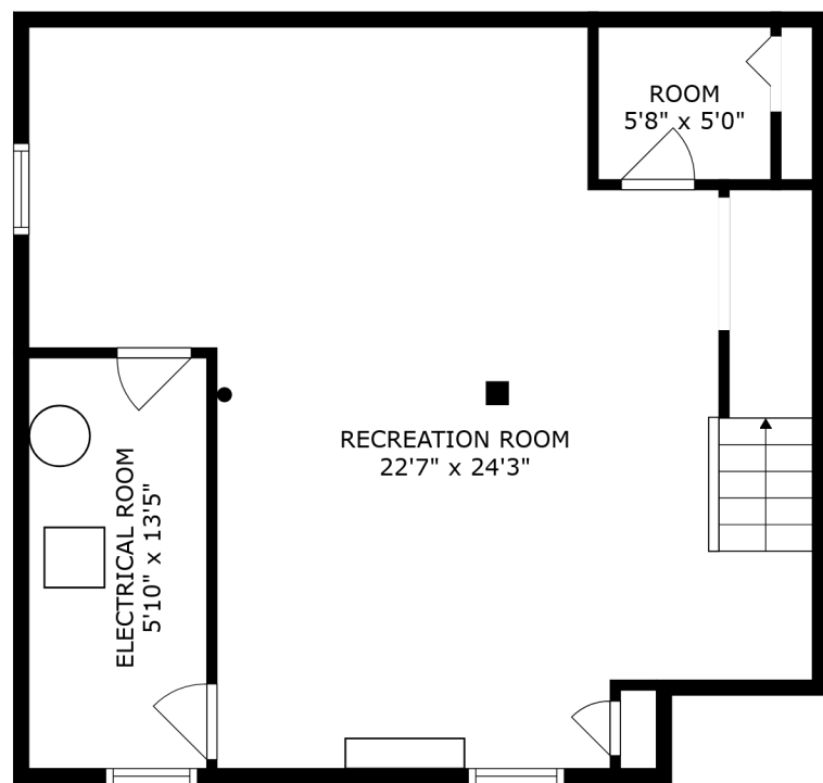
FLOOR 1
