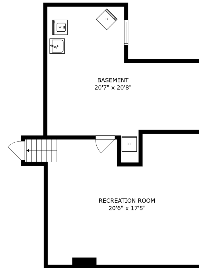
FLOOR 1
