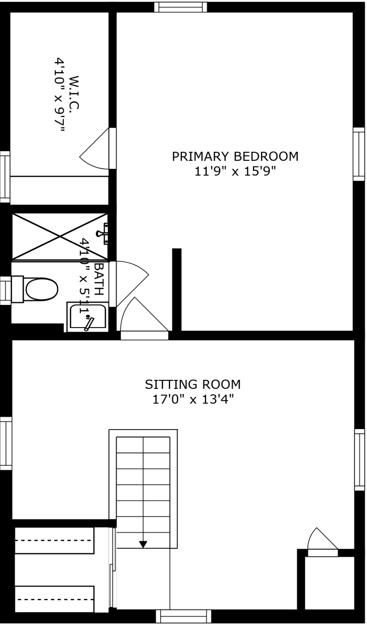
FLOOR 3
