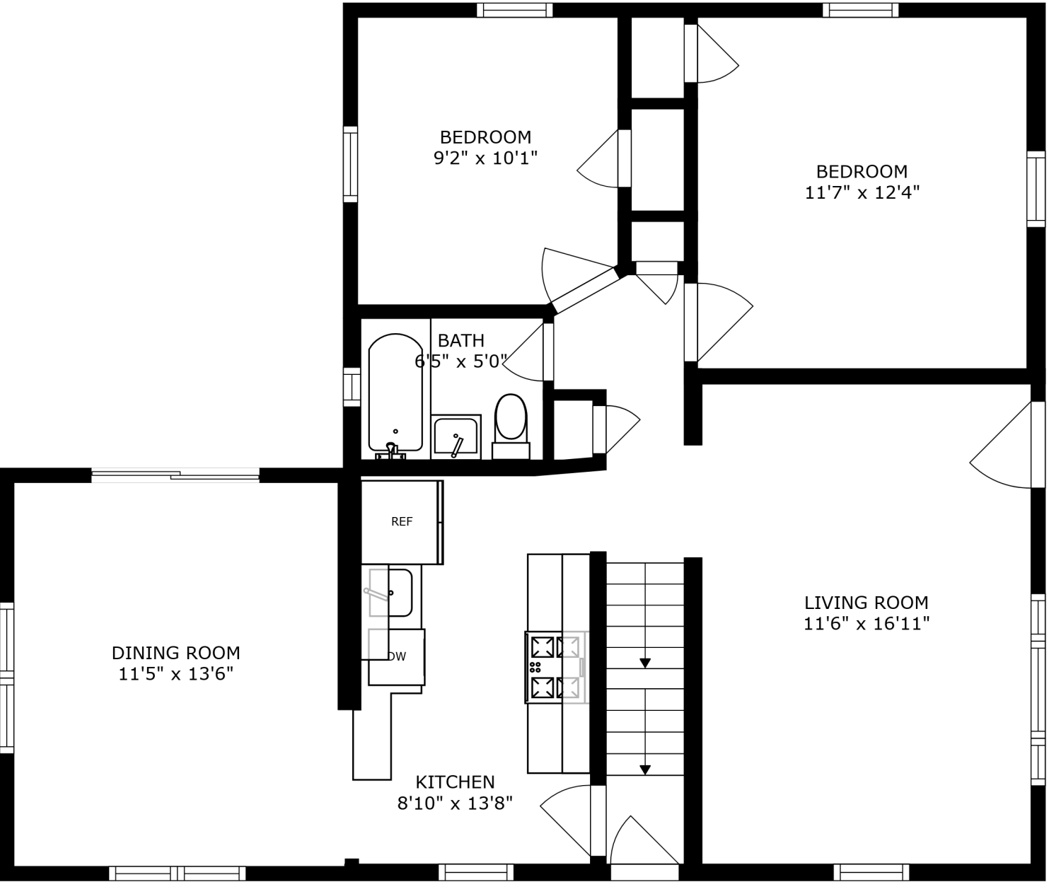
FLOOR 2
