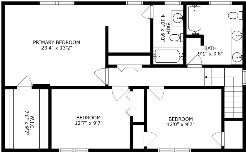
FLOOR 3
