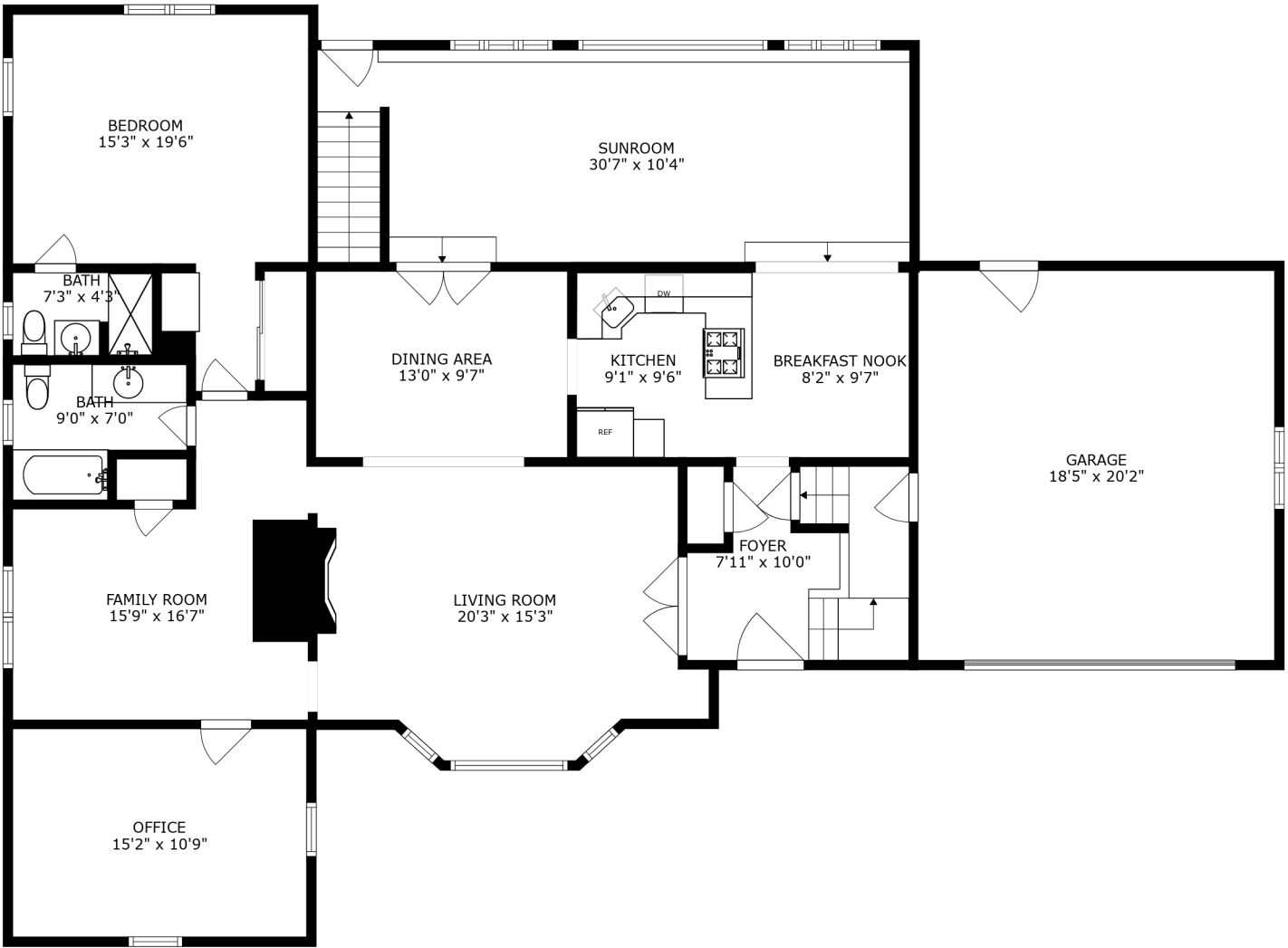
FLOOR 2
