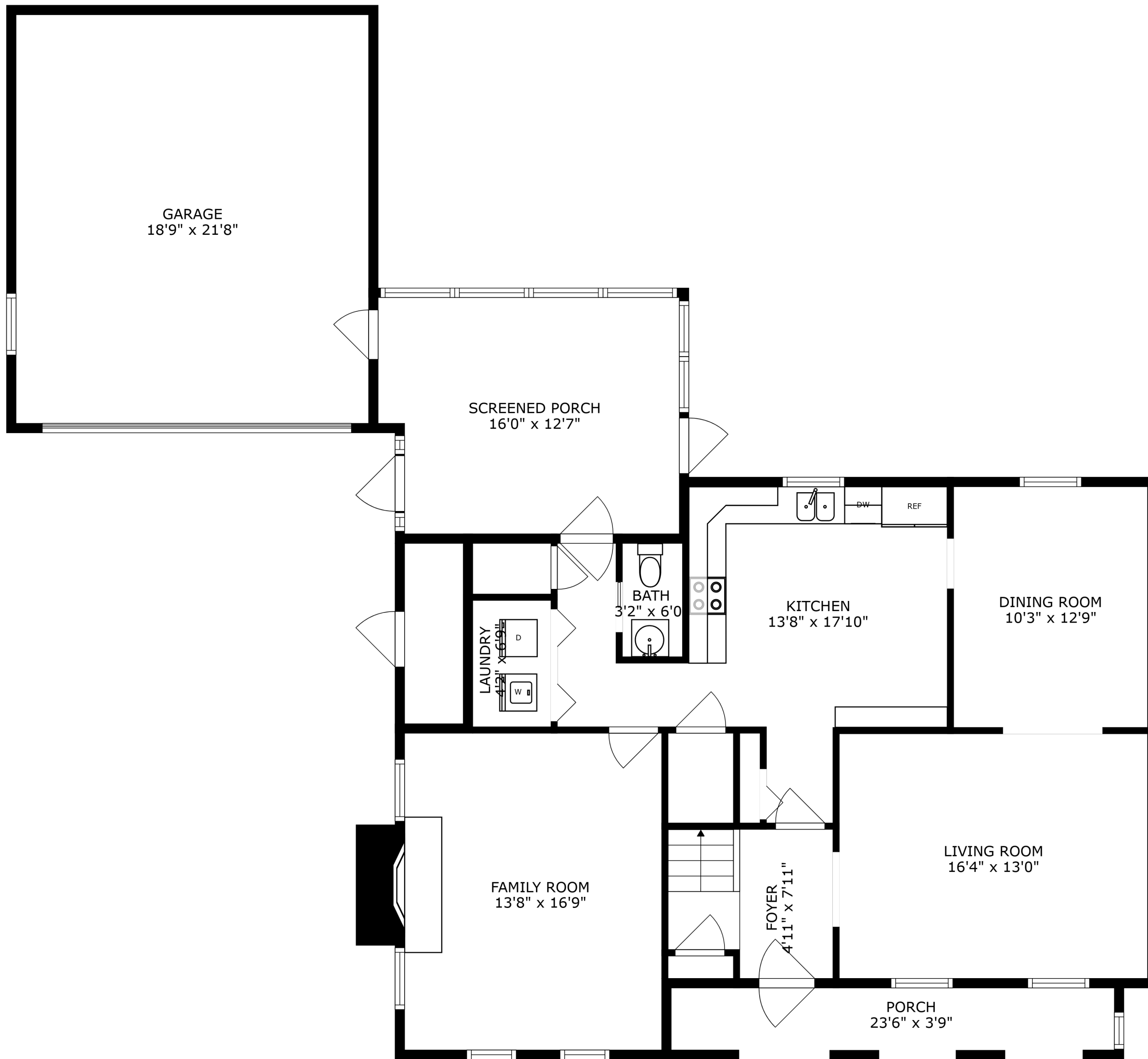
FLOOR 1
