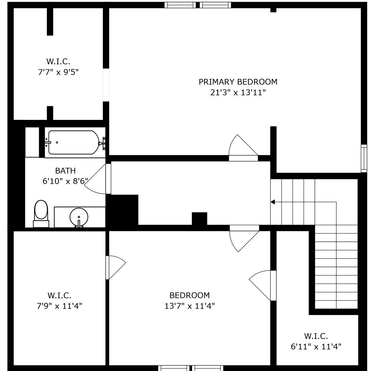
FLOOR 3
