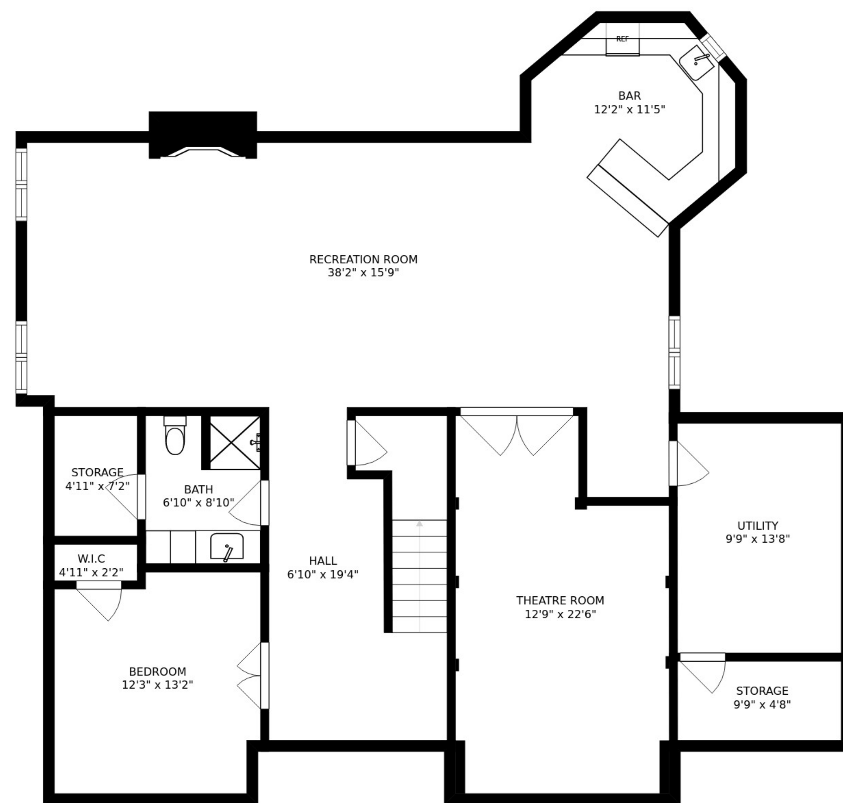
FLOOR 1
