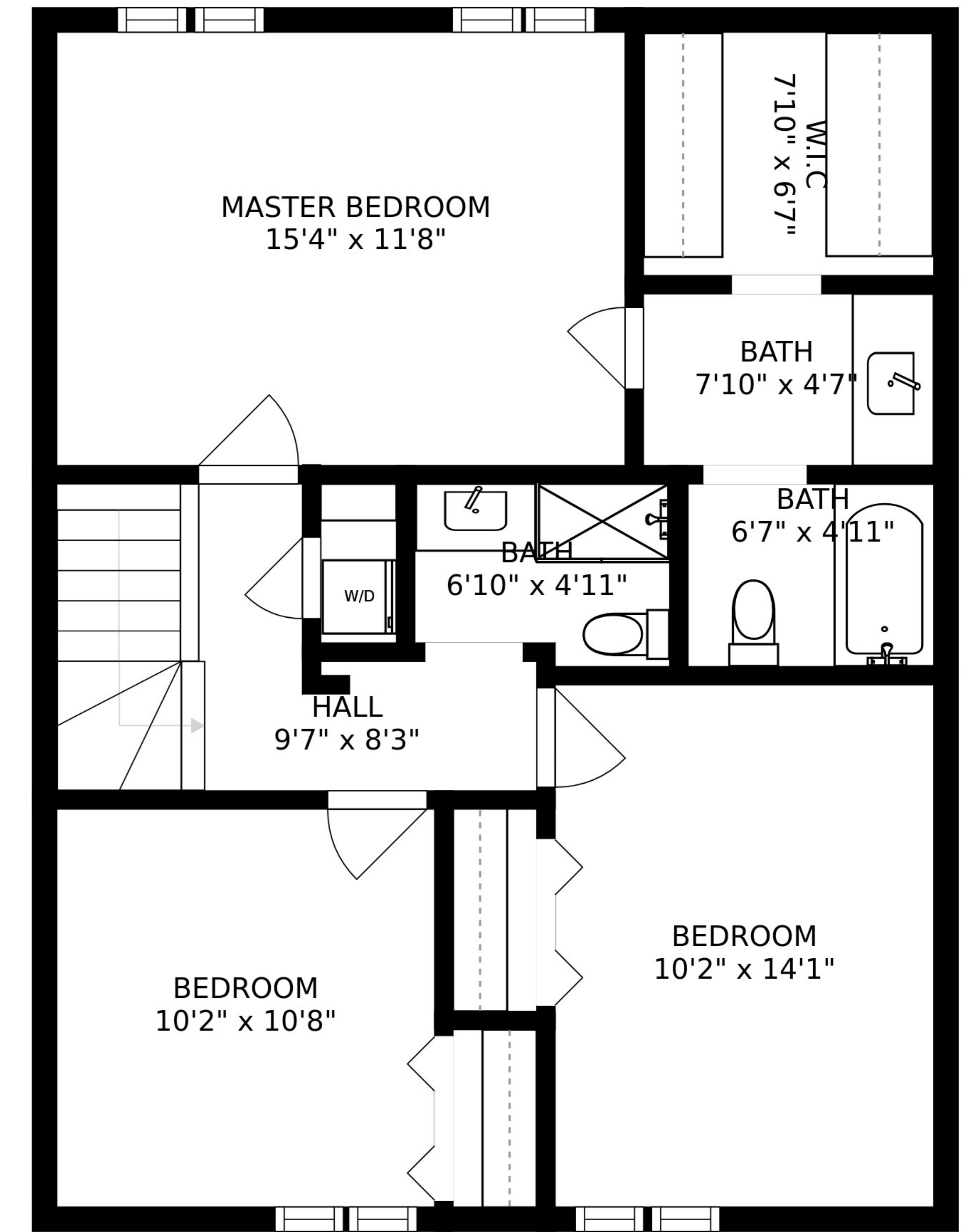
FLOOR 3
