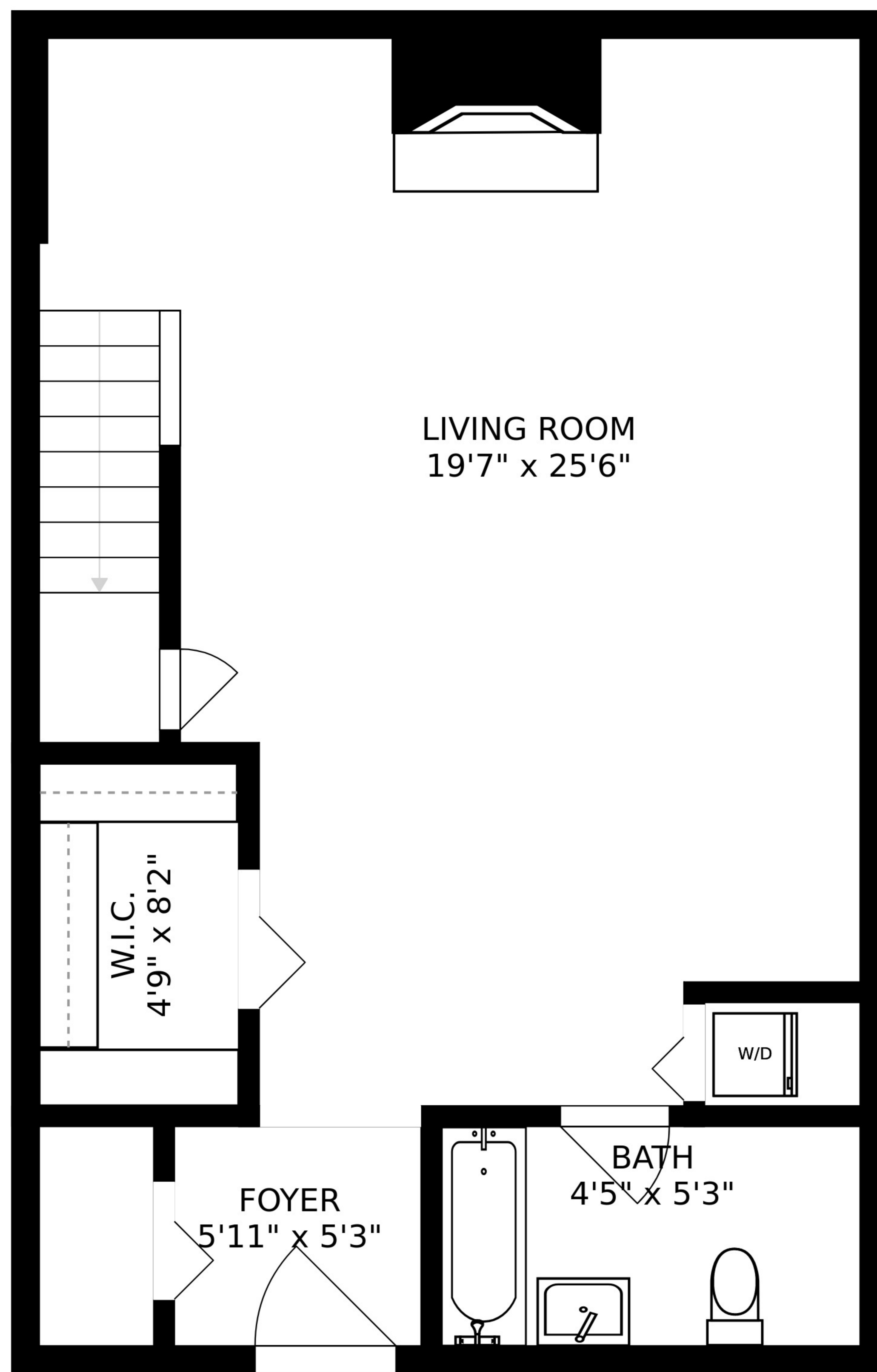
FLOOR 1
