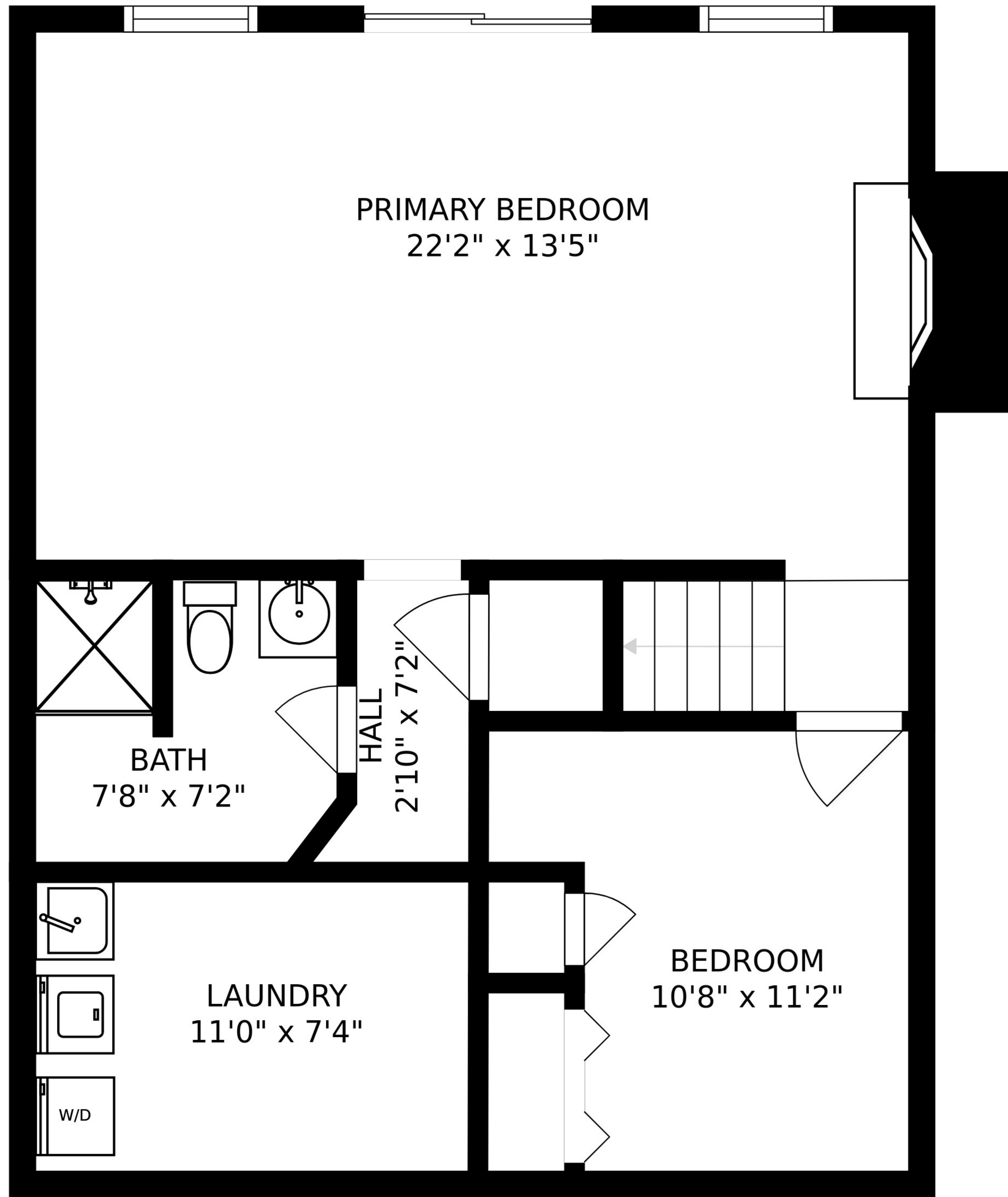
FLOOR 1
