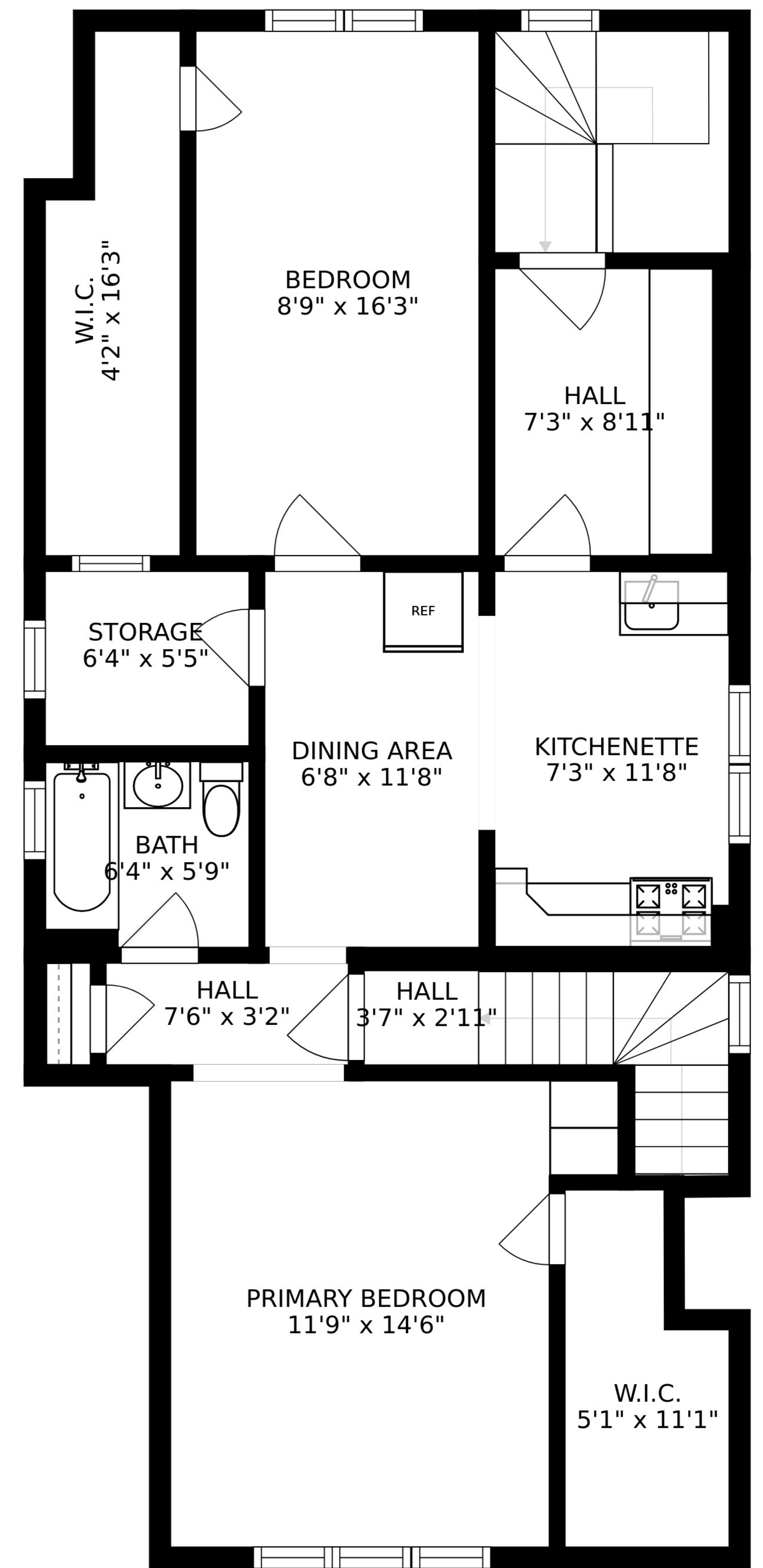
FLOOR 3
