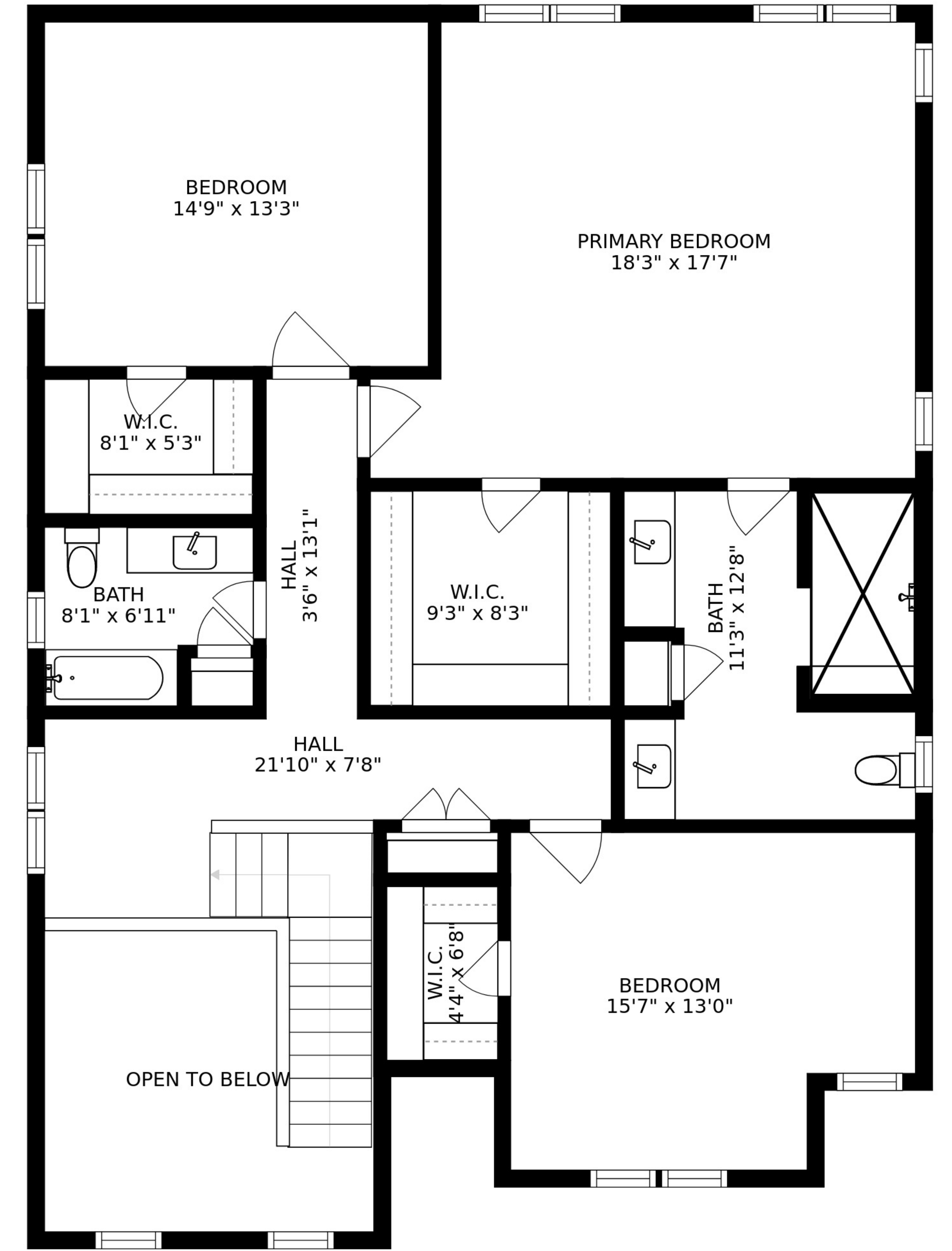
FLOOR 3
