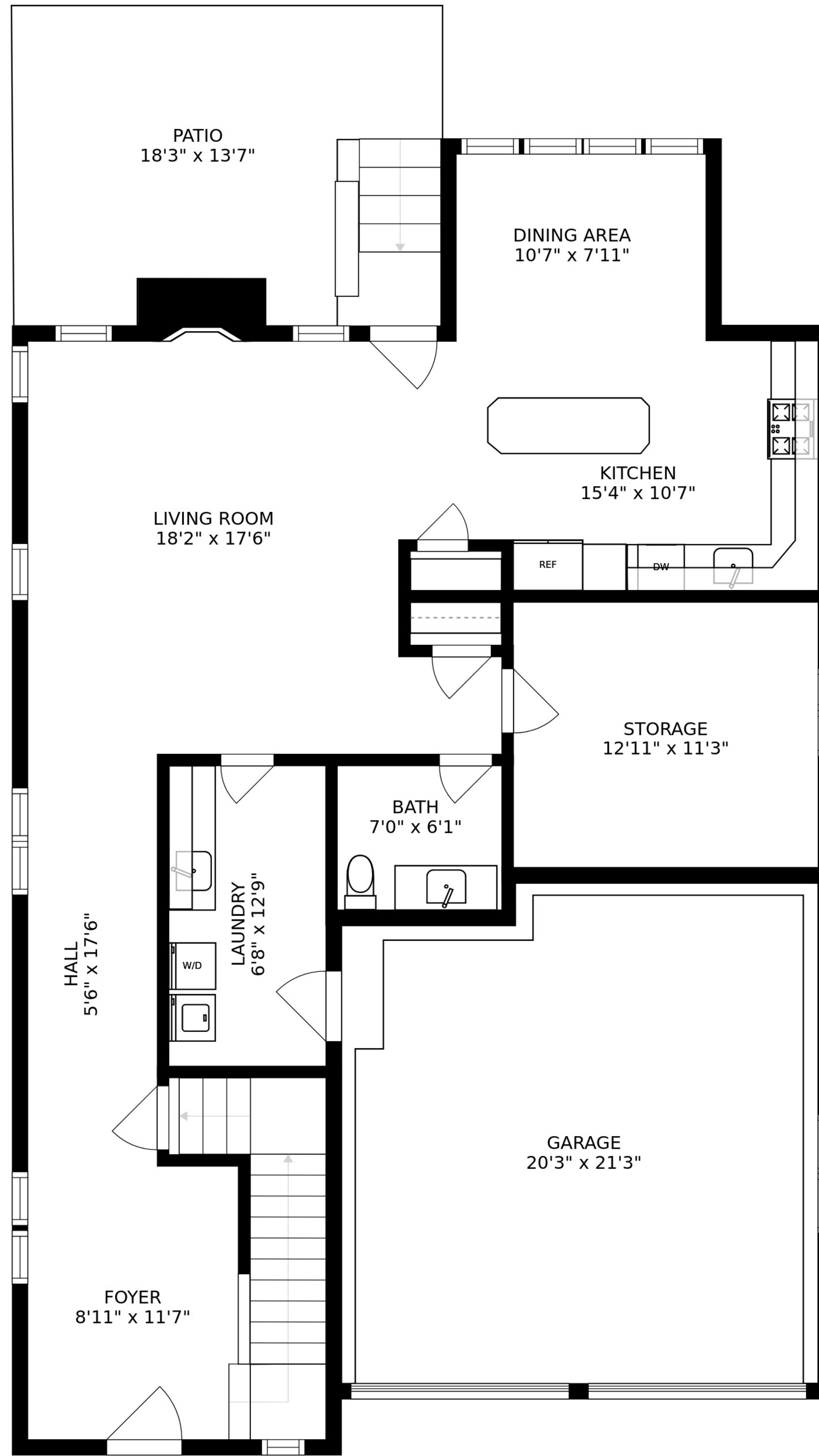
FLOOR 2
