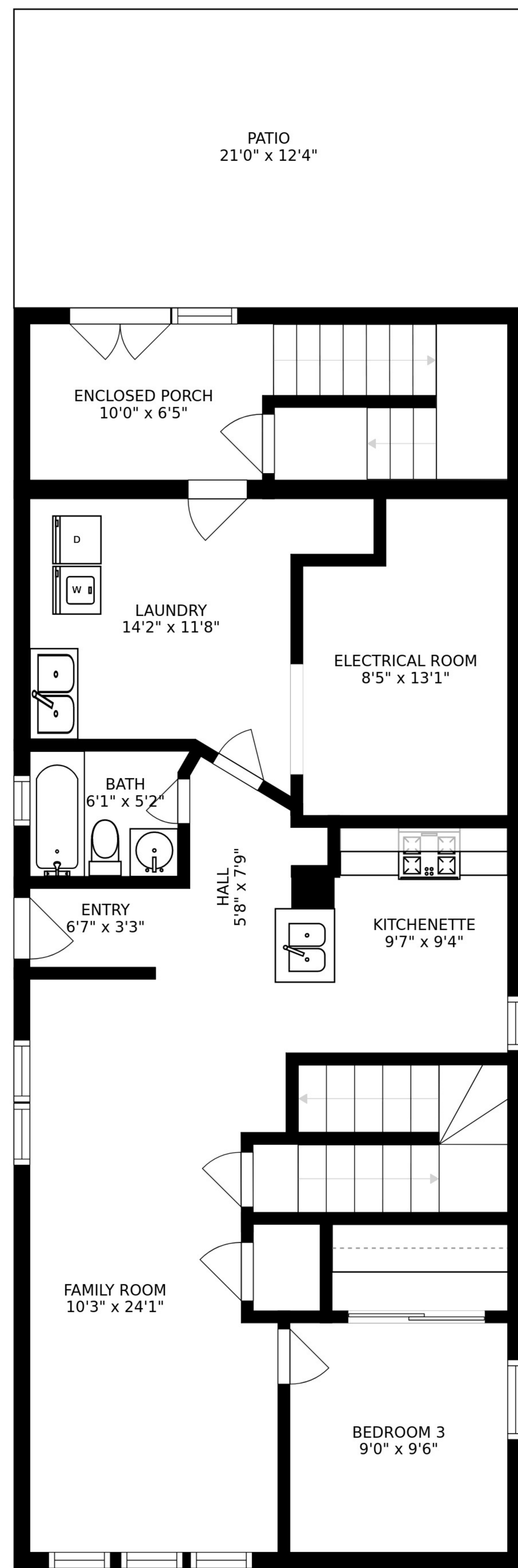
FLOOR 1
