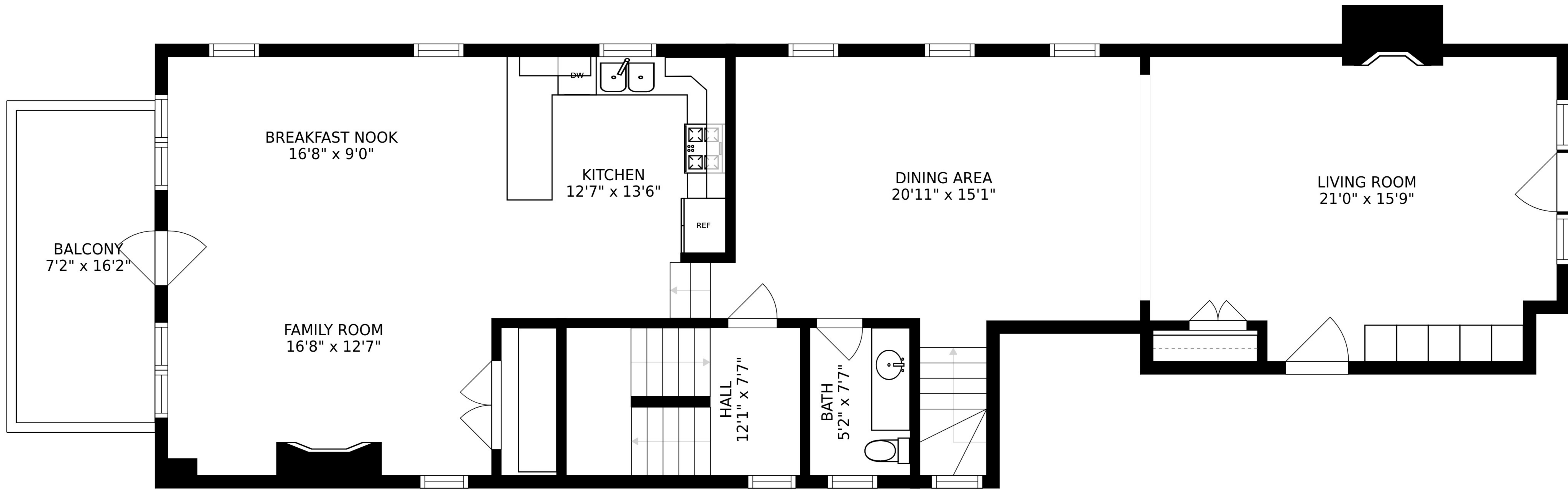
FLOOR 2
