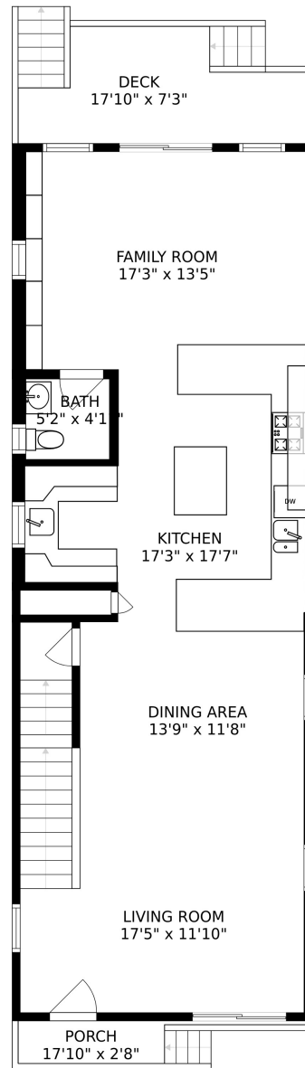
FLOOR 2
