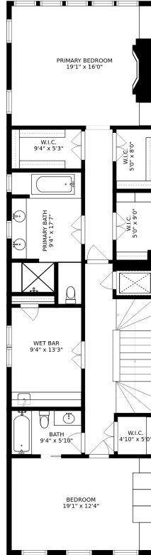
FLOOR 3
