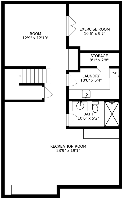
FLOOR 1
