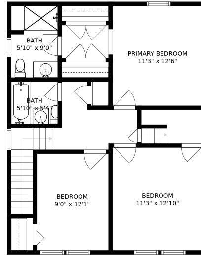
FLOOR 3
