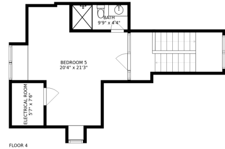
FLOOR 4
