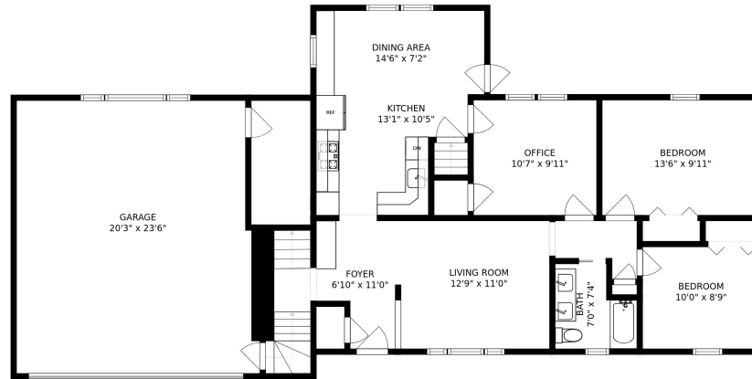
FLOOR 2
