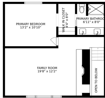
FLOOR 3
