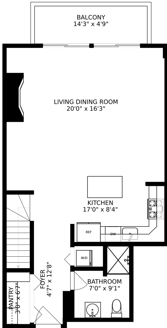
FLOOR 1
