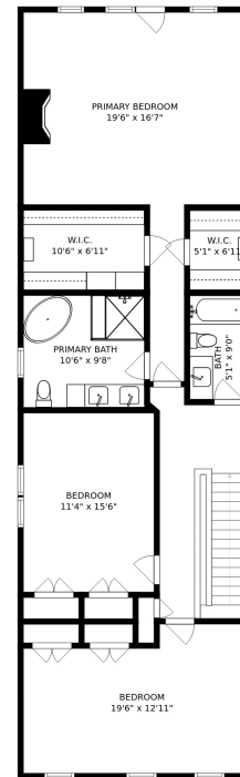
FLOOR 3
