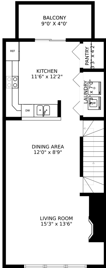
FLOOR 2
