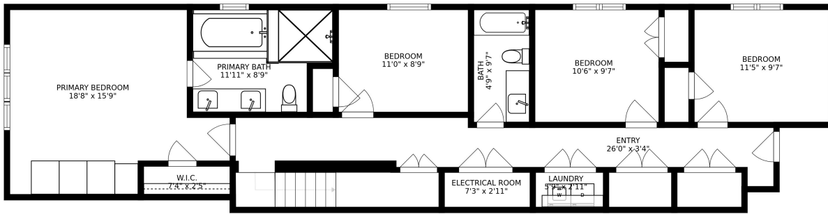
FLOOR 1
