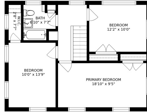
FLOOR 3
