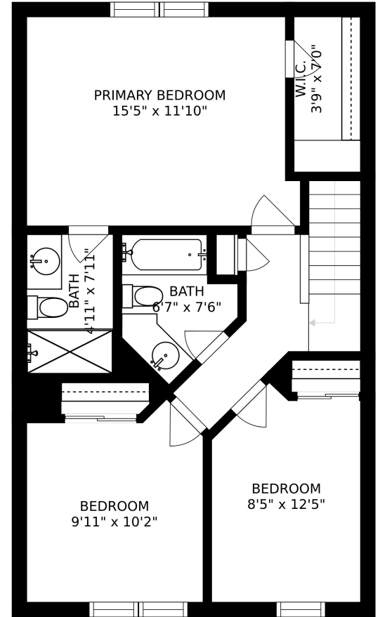
FLOOR 3
