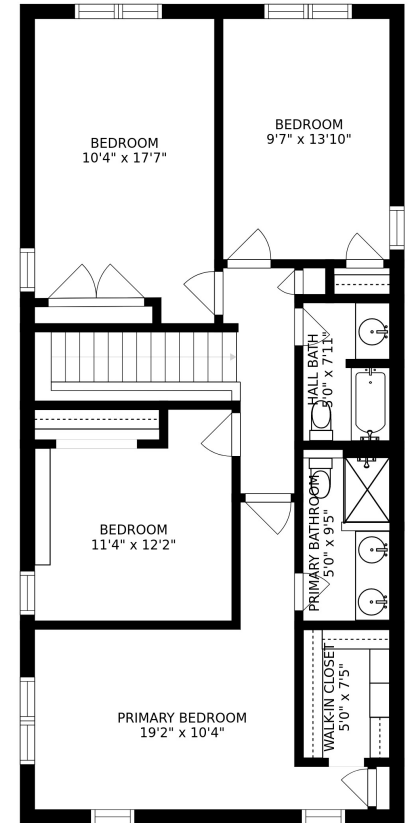
FLOOR 3
