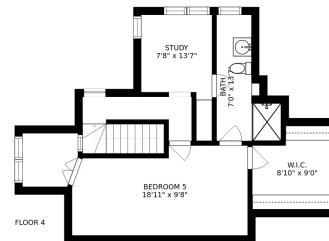
FLOOR 4
