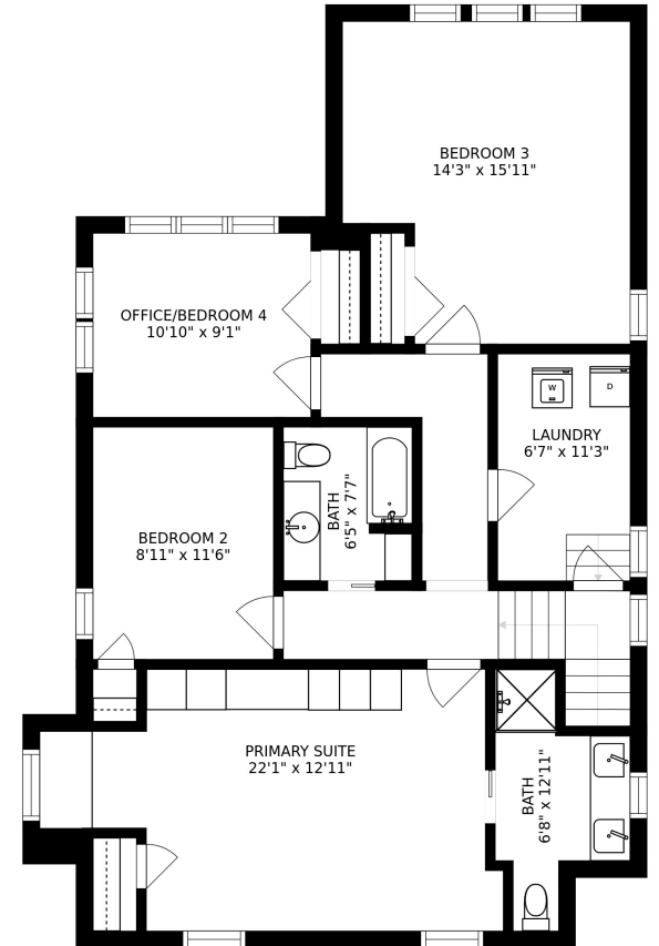
FLOOR 3
