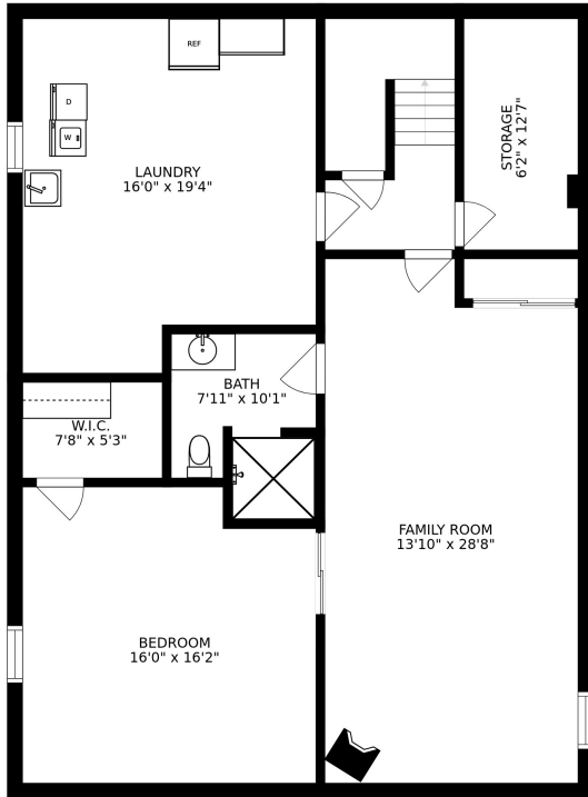
FLOOR 1
