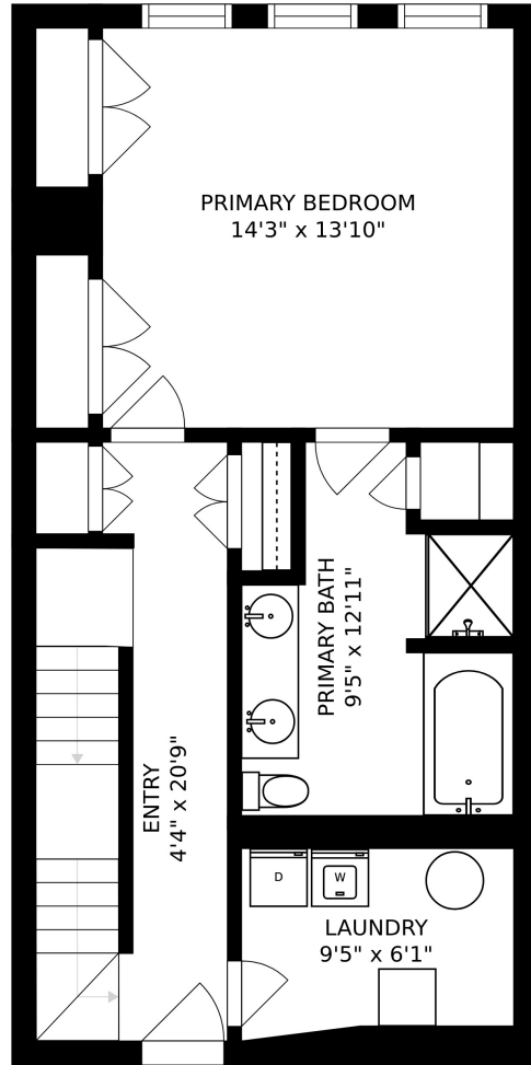
FLOOR 2
