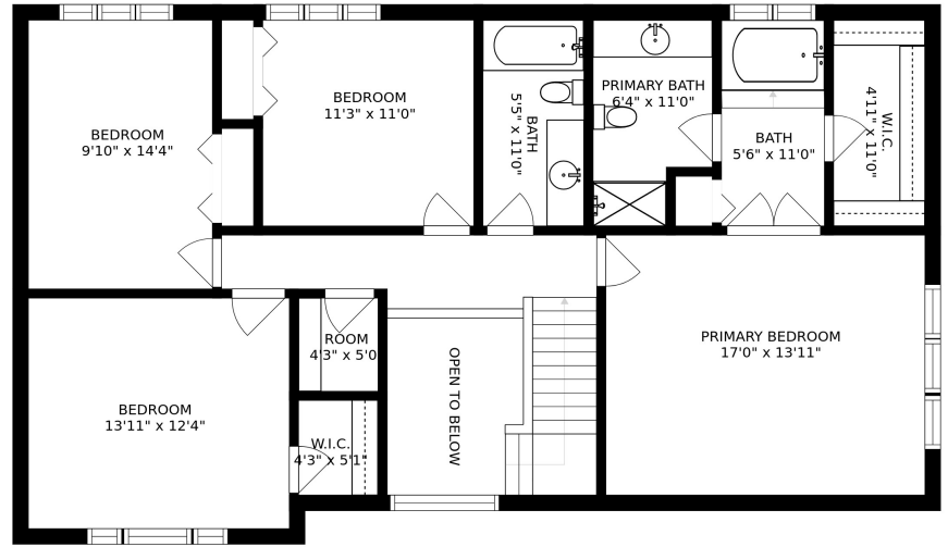
FLOOR 3
