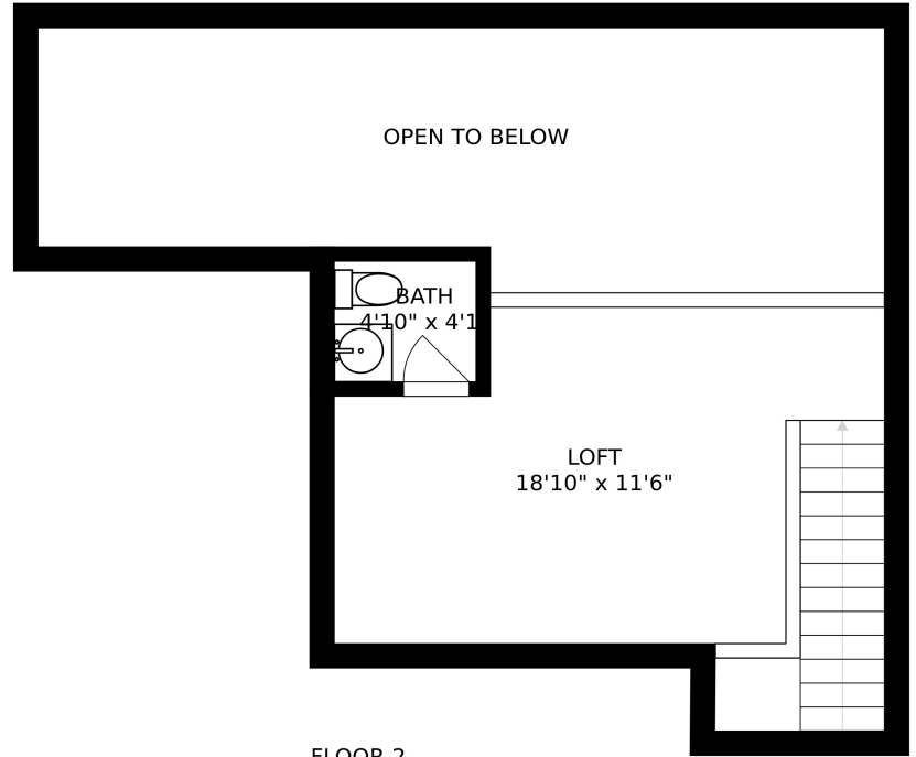
FLOOR 2
