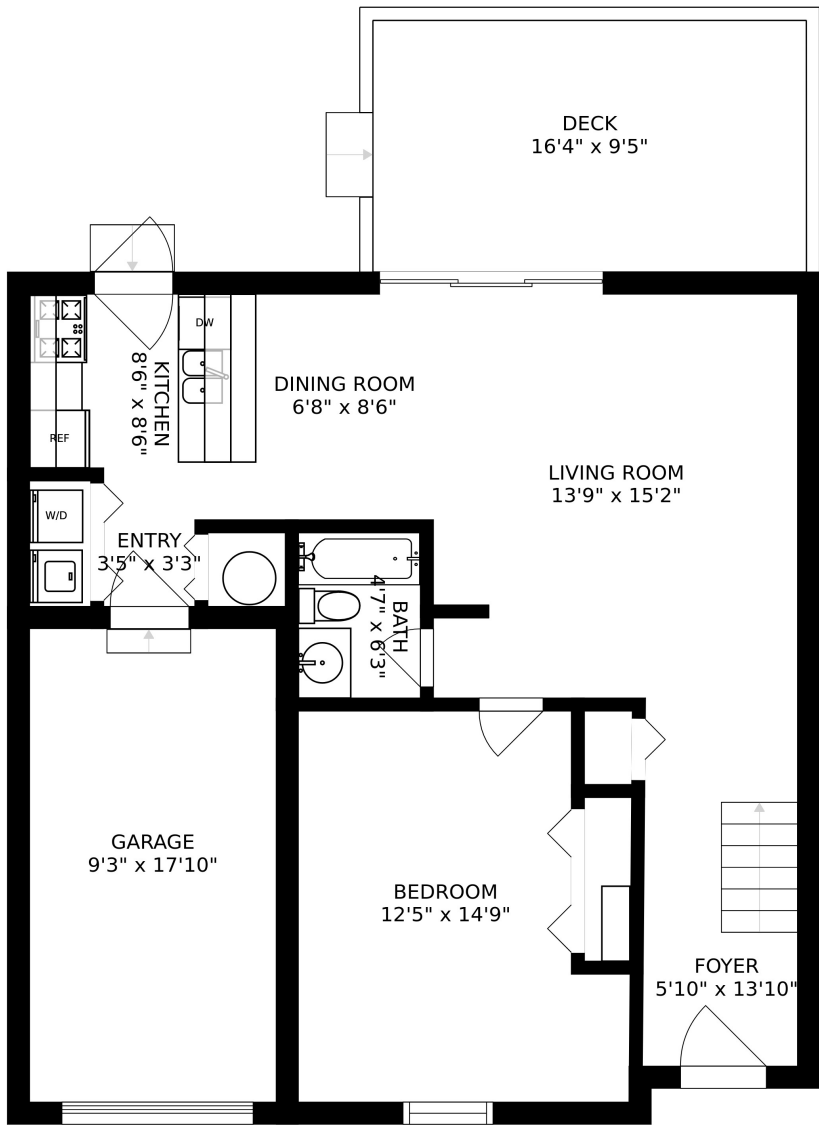
FLOOR 1
