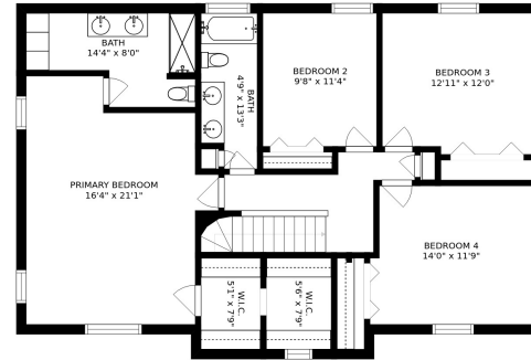
FLOOR 3
