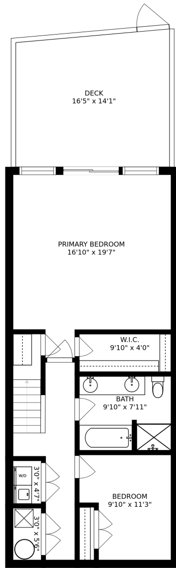
FLOOR 1
