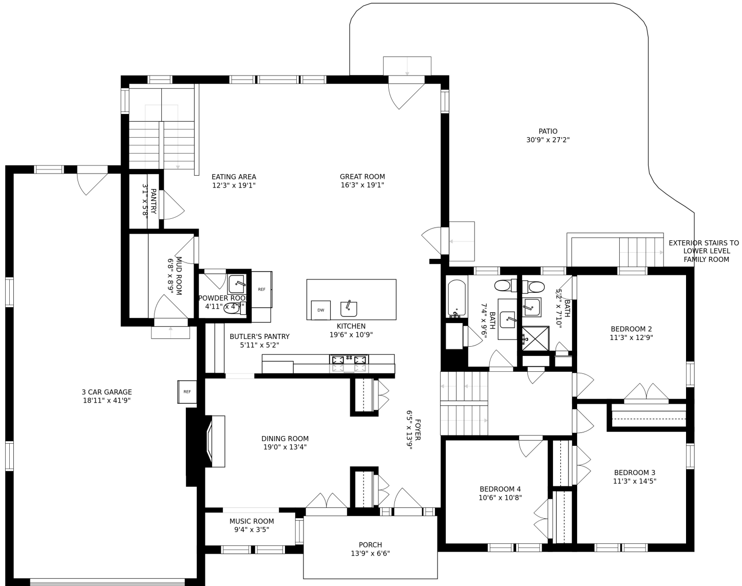
FLOOR 1
