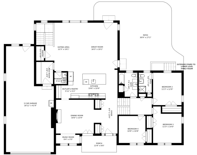
FLOOR 1
