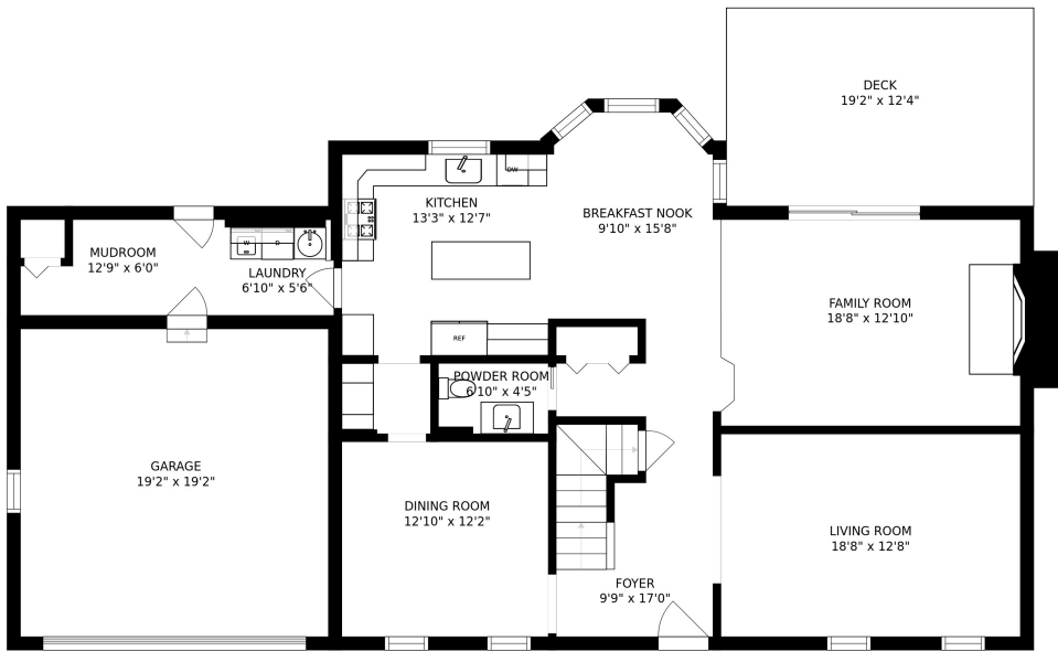
FLOOR 2
