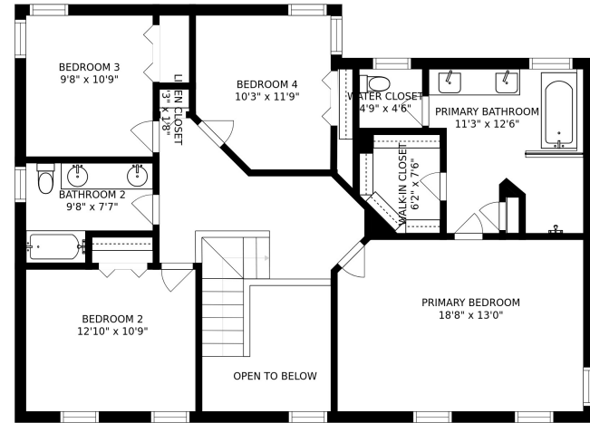
FLOOR 3
