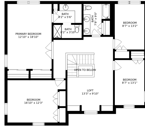
FLOOR 3
