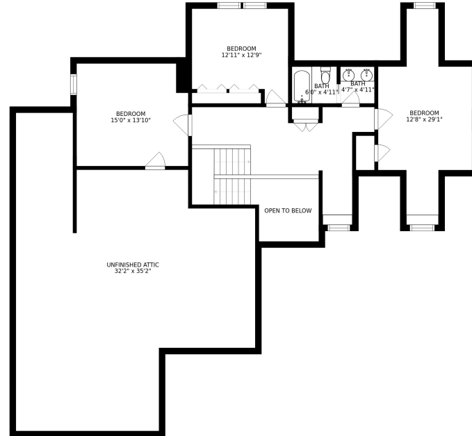
FLOOR 3
