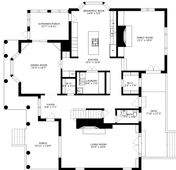
FLOOR 2
