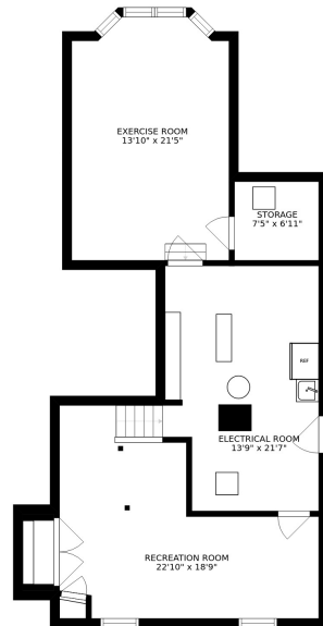
FLOOR 1
