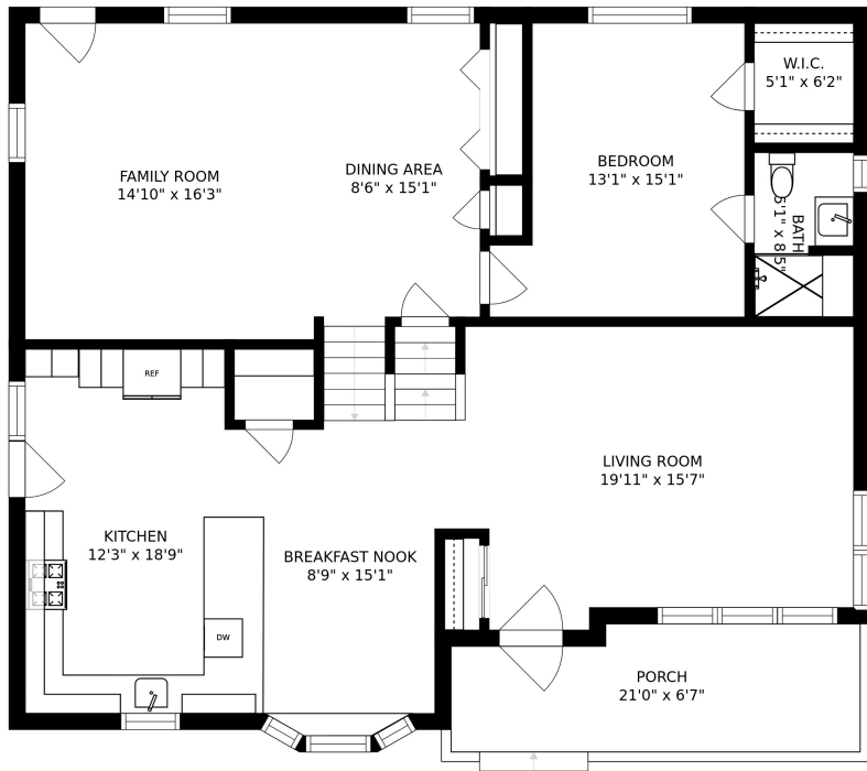
FLOOR 2
