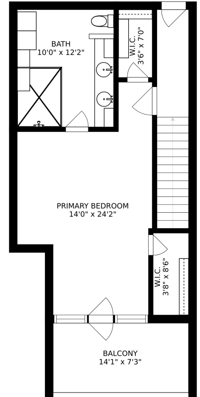
FLOOR 4
