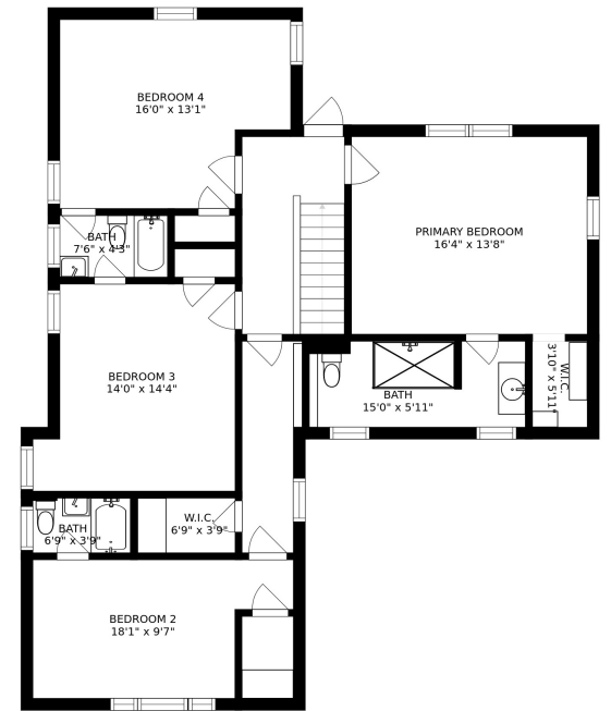
FLOOR 3
