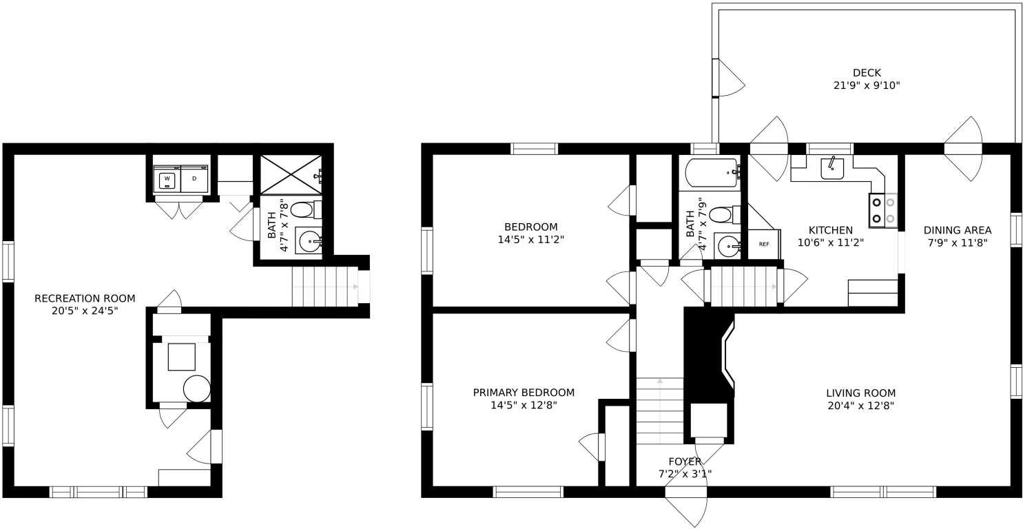
FLOOR 1
