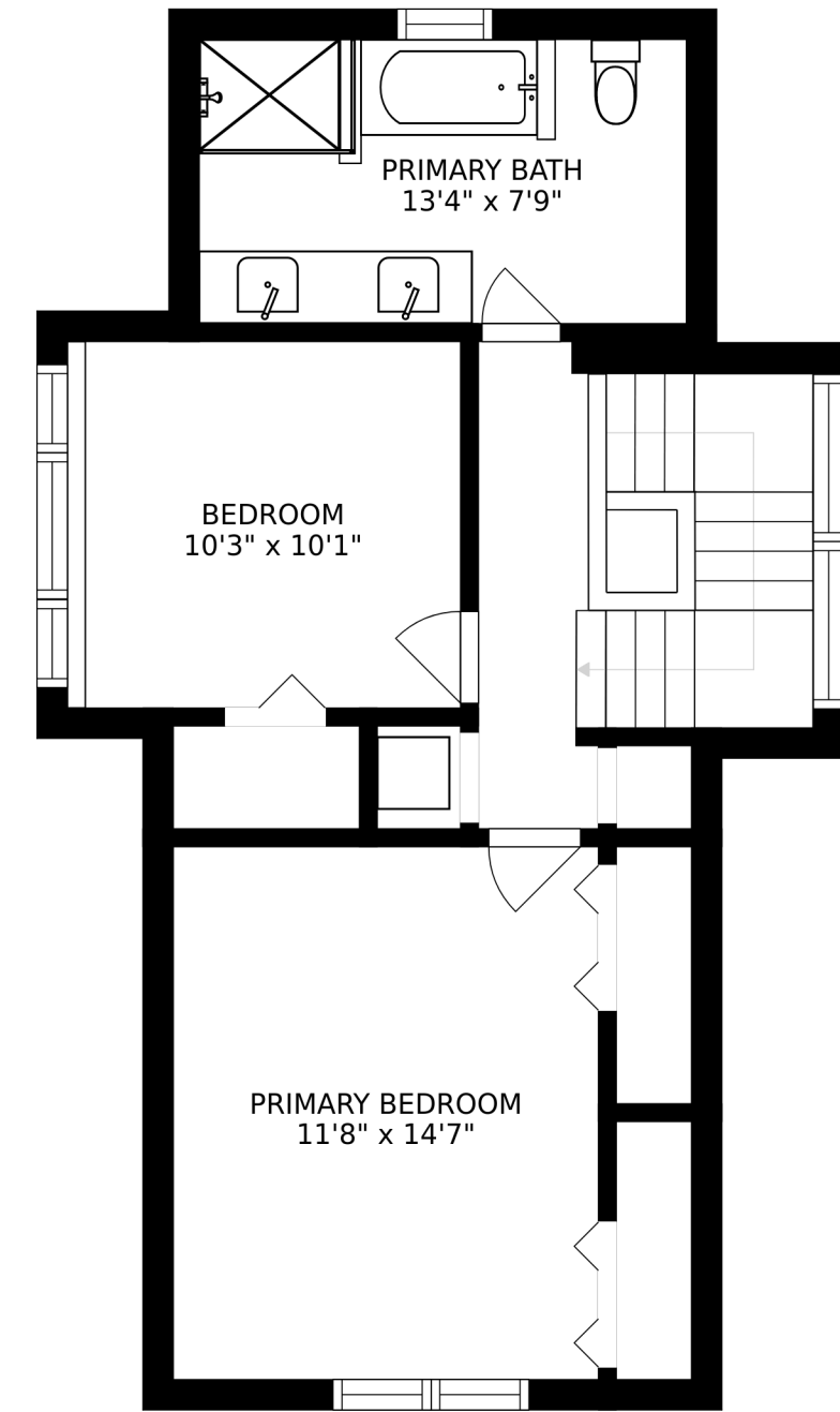
FLOOR 3
