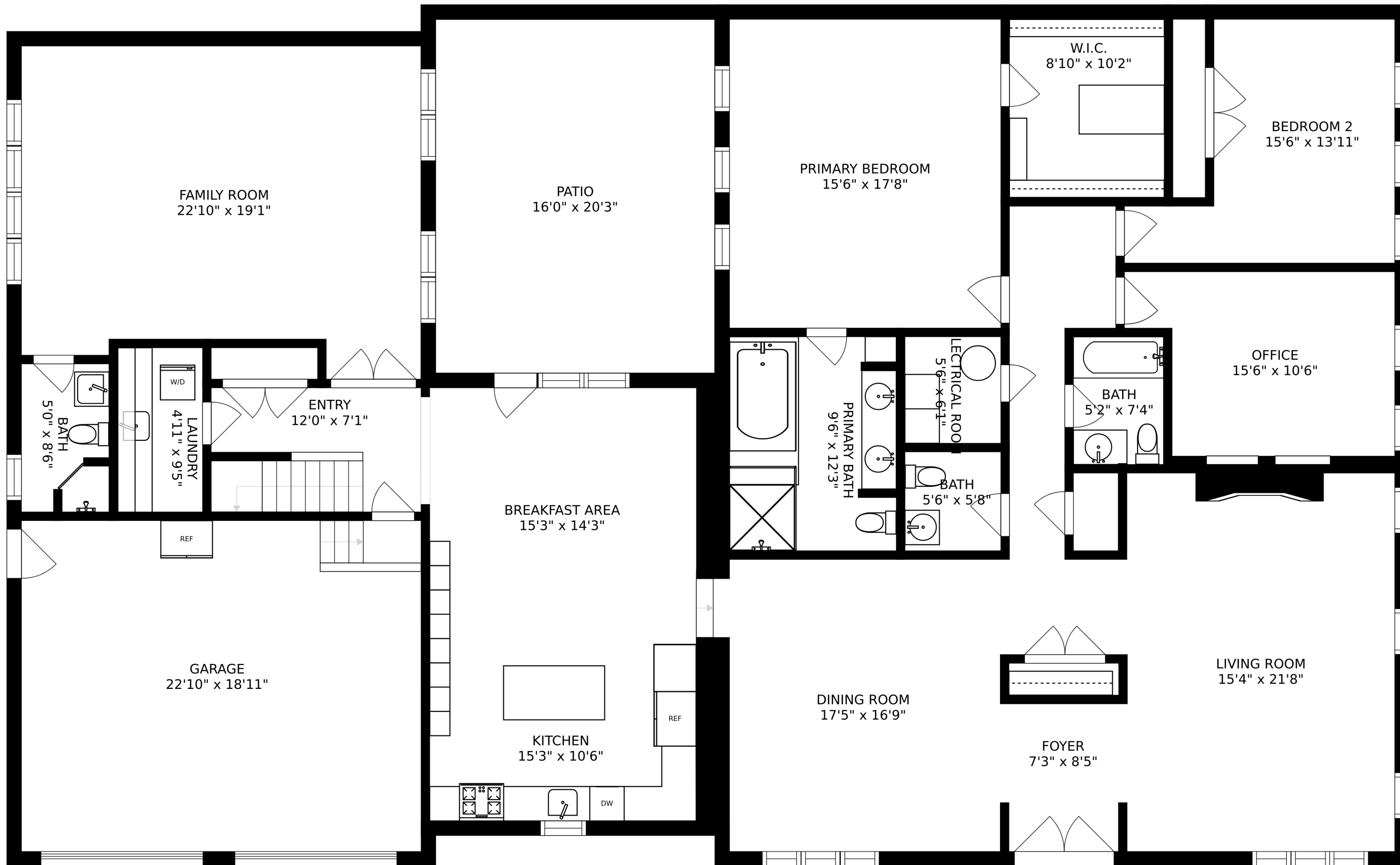
FLOOR 1
